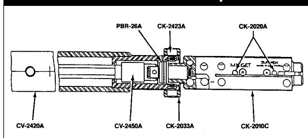
CV-2405A Midget Hone Head
